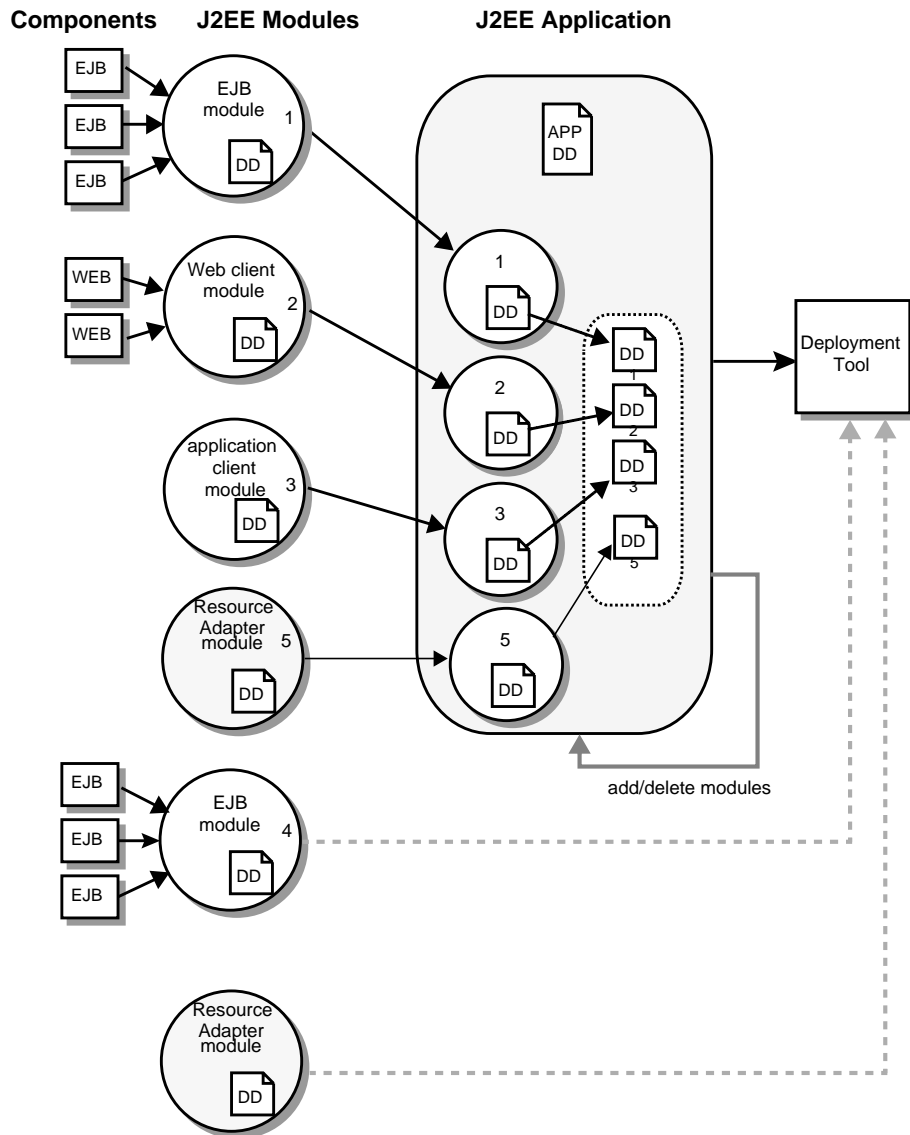
FIGURE 8-1 J2EE Deployment
