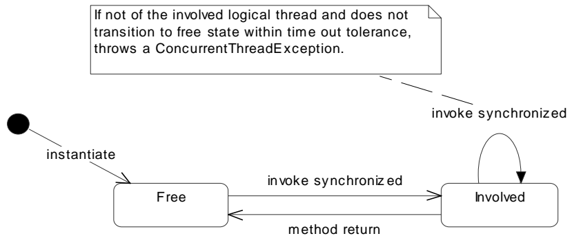
Figure 17. State Diagram of Object Methods Synchronized with Respect to Logical Threads.
