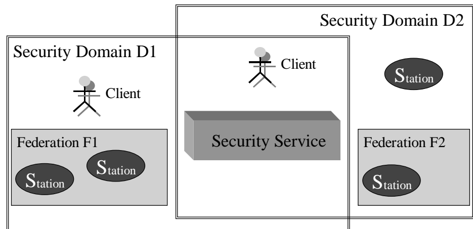
Figure 12. Security Architecture.
