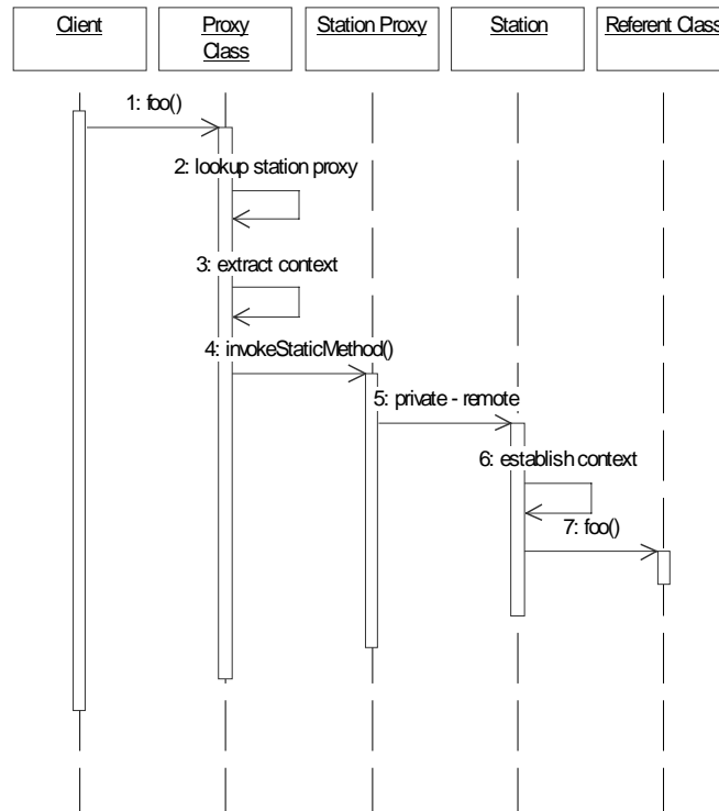
Figure 8. Referent Class Method Invocation.
