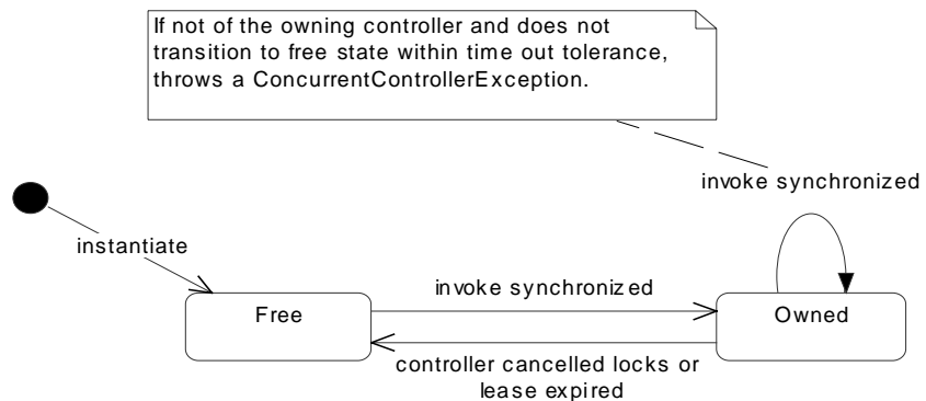
Figure 18. State Diagram of Object Methods Synchronized with Respect to Controllers.
