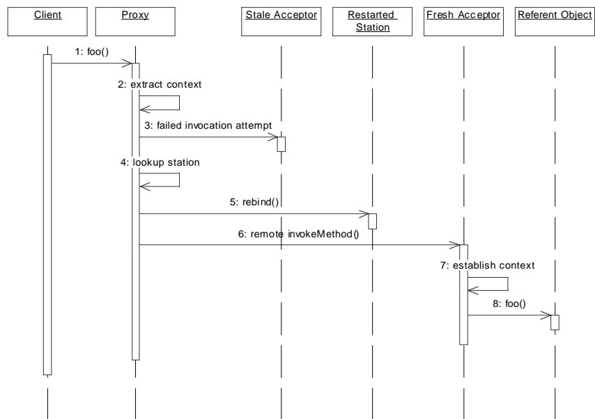
Figure 11. Proxy Rebinding.
