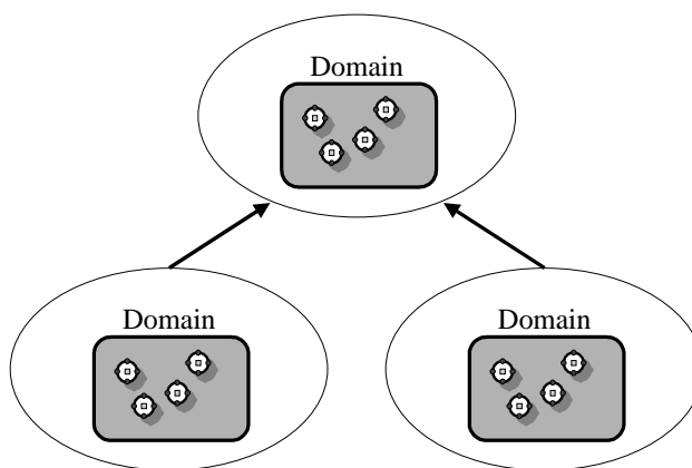
Figure 3. Interdomain Federation.
