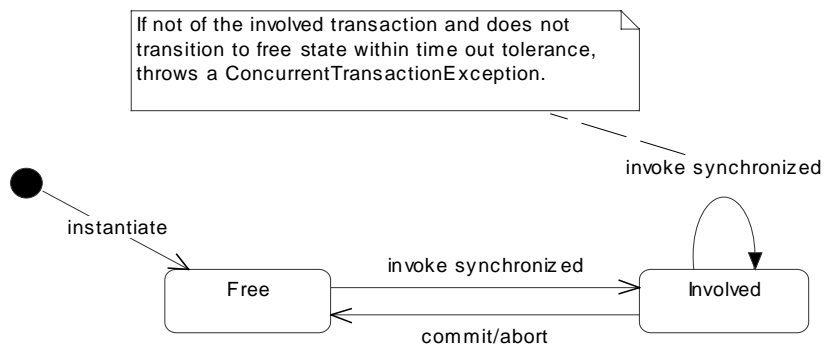
Figure 16. State Diagram of Object Methods Synchronized with Respect to Transactions.
